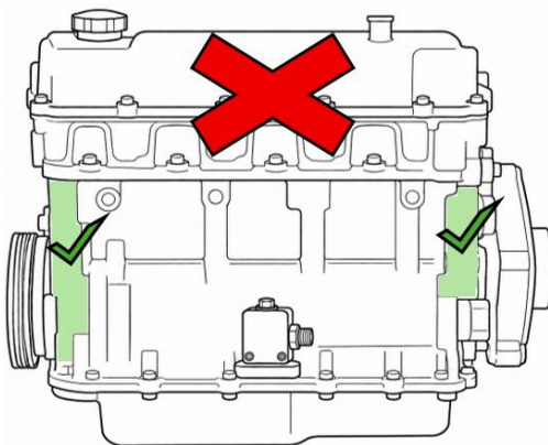
Fig. 16 Accelerometer placement
